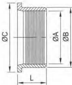
RJT Expanding Liner RJT-14R
