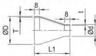
SMS SMS Concentric Reducer
