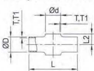
SMS Welding Cross Without Straight-End
