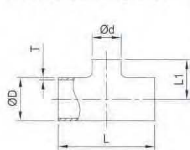
Long Reducing Tee
