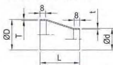
SMS SMS Eccentric Reducer
