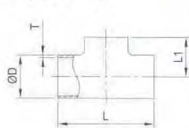
Welding Tee
