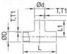
SMS Tee Without Straight-End
