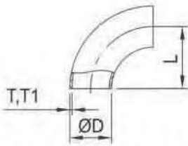
SMS 90 B 90° Short Elbow
