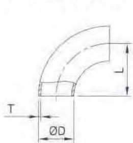
90° Short Bend C.2WCL-90° Bend
