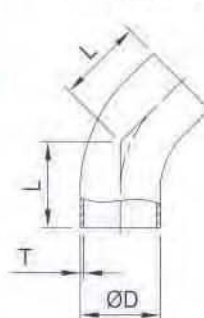
45° Long Elbow C.L2KS-45° Elbow
