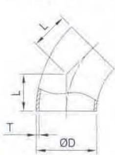
45° Short Elbow C.2WK-45° Elbow
